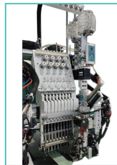
2色散珠装置 2 Colors Beading Device
